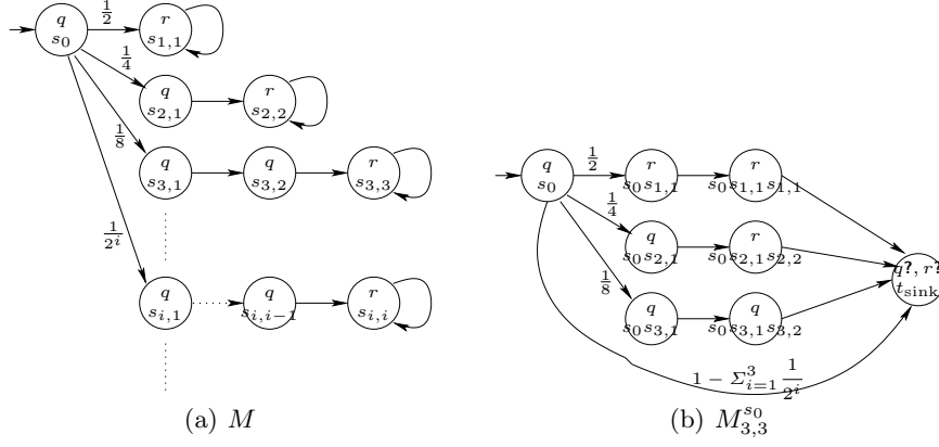
Fig. 2. A model M satisfying [\mathbf{qU}\mathbf{r}]_{\geq 1} and [\mathbf{qW}\mathbf{r}]_{\geq 1} , and its unfolding M_{3,3}^{s_0}
